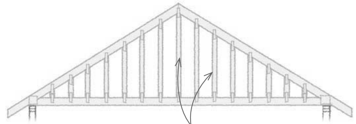
Vertical pieces provide the required nailing for sheathing and siding.
