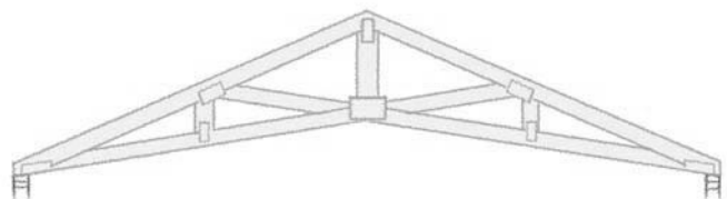
A drop-top truss supports the rake boards.
